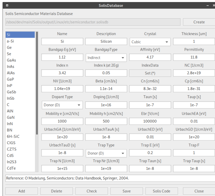
Figure 3.12: SolisDatabase Screenshot.
