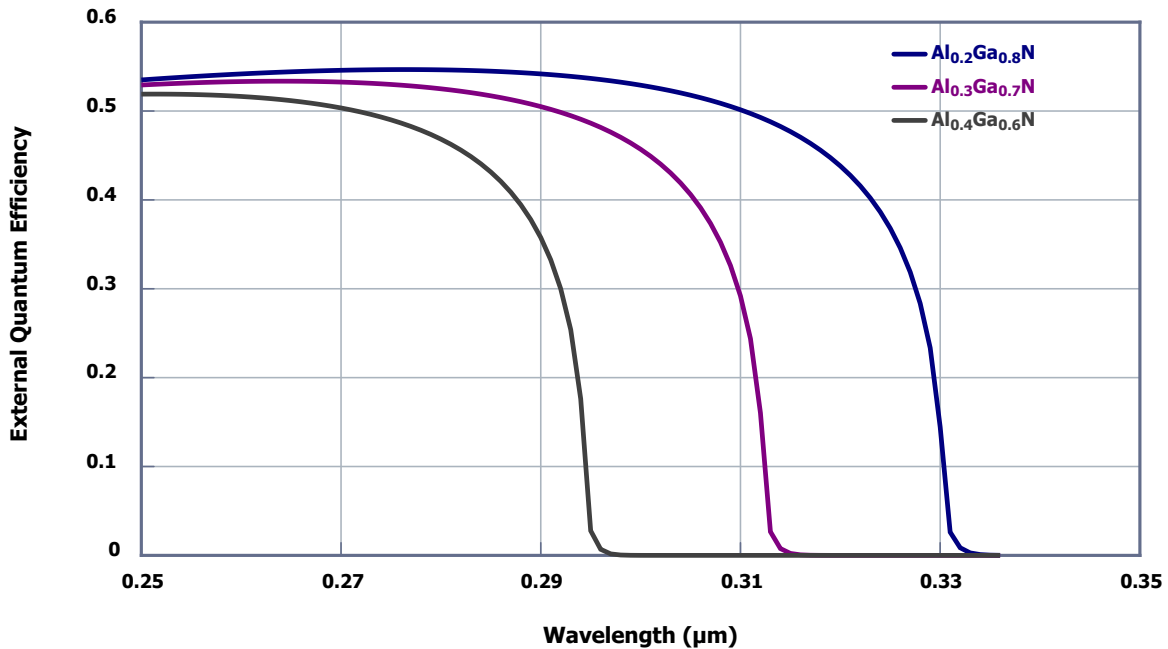
Figure 4.6: The AlGa x N Schottky UV detector external quantum efficiency spectrum for three aluminum composition x in Al x Ga 1- x N. The corresponding Solis input code is shown in Listing 4.9.
