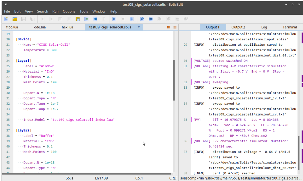
Figure 3.1: SolisEdit Screenshot.
