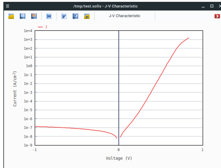
Figure 3.11: SolisPlot Screenshot.
